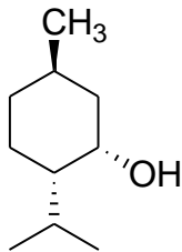
neomenthol (found in peppermint oil)
