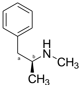
methamphetamine
