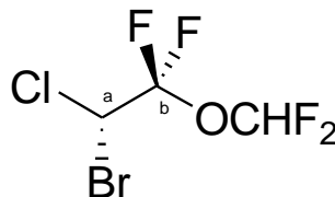
enflurane (a general anesthetic)
